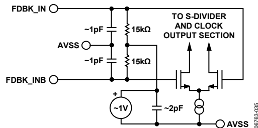
Figure 43. Differential FDBK Inputs
