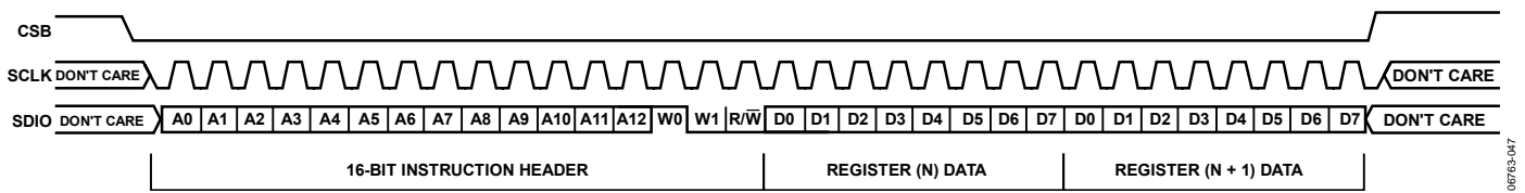
Figure 55. Serial Control Port Write—LSB First, 16-Bit Instruction, 2 Bytes Data
